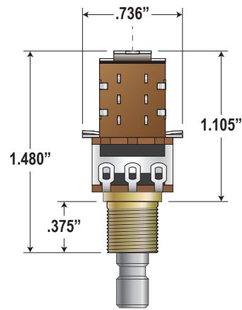
Typical Non-Solderless Bourns Push/Pull
