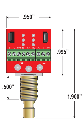
ToneShapers Solderless CTS Push/Pull (PP01)
