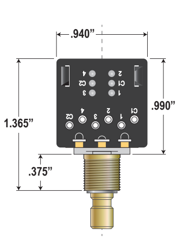
Typical Non-Solderless CTS Push/Pull
