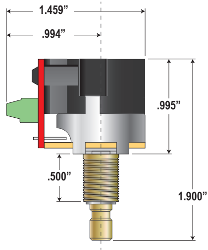
ToneShapers Solderless CTS Push/Pull (PP01)
