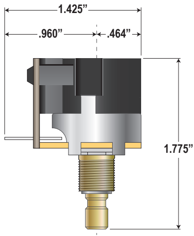
Typical Non-Solderless CTS Push/Pull
