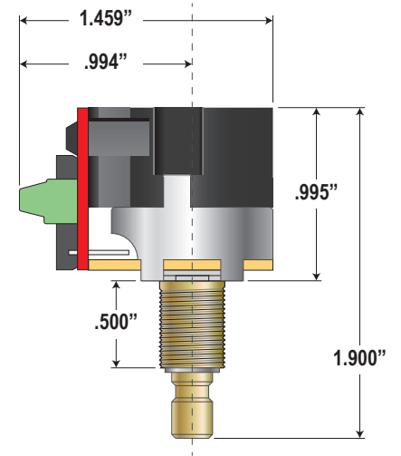
ToneShapers Solderless CTS Push/Pull (PP02)
