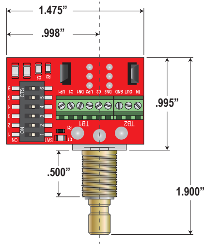
ToneShapers Solderless CTS Push/Pull (PP02)
