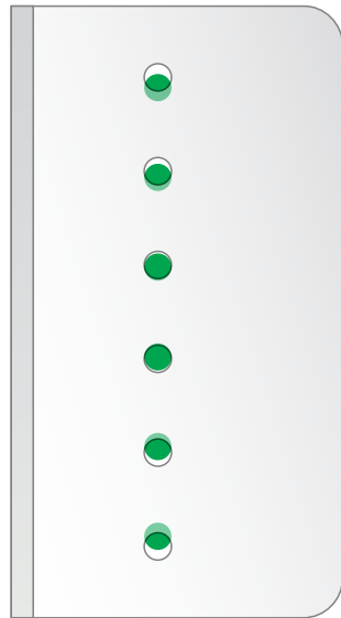
Bridge plate drawn with 2-7/32" hole spacing. Green circles are on 2-1/8" centers.
