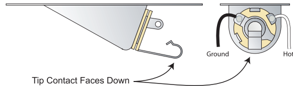
Jack Detail
